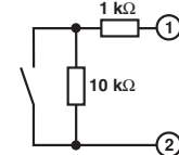
Figure 6 Switch contact with resistance circuit
